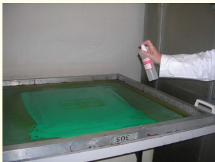
Step 1. Spray SS-350 on squeegee side of screen.
